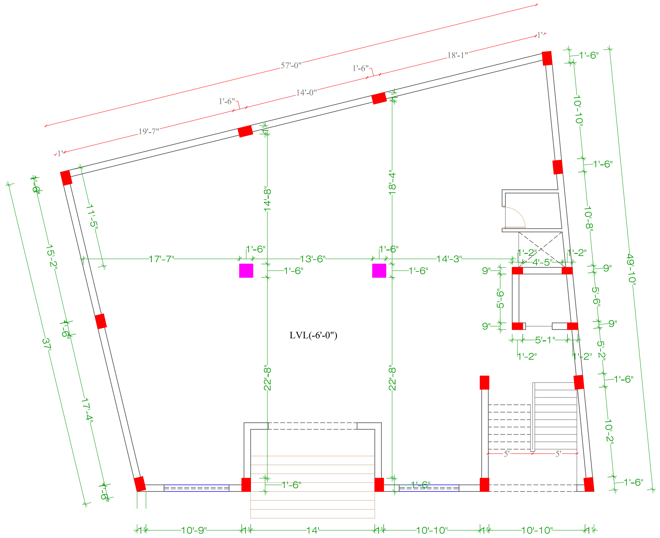
COLUN CENTER LINE PLAN
